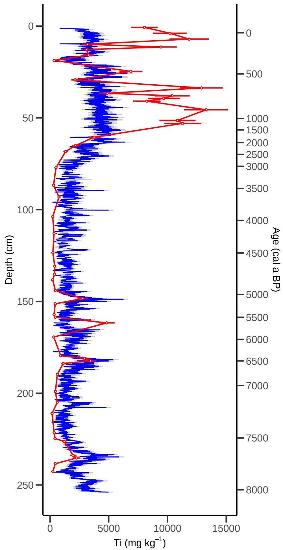
KER1: PLSR Ti Predictions with Confidence Intervals
